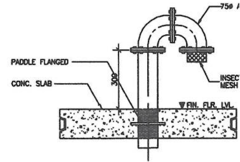
(IN R.C. SLAB) DETAIL OF AIRVENT P
