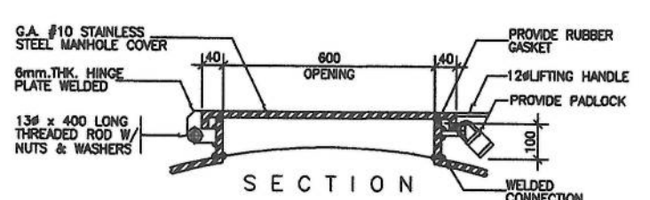
DETAIL OF MANHOLE COVER (FOR STAINLESS STEEL WATER TANK) 2 SCALE N D T S
