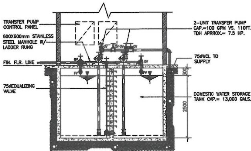
SECTION - 'A'
