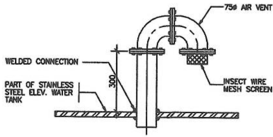
(IN STAINLESS STEEL) 1 DETAIL OF AIRVENT PIPE SCALE N D T S
